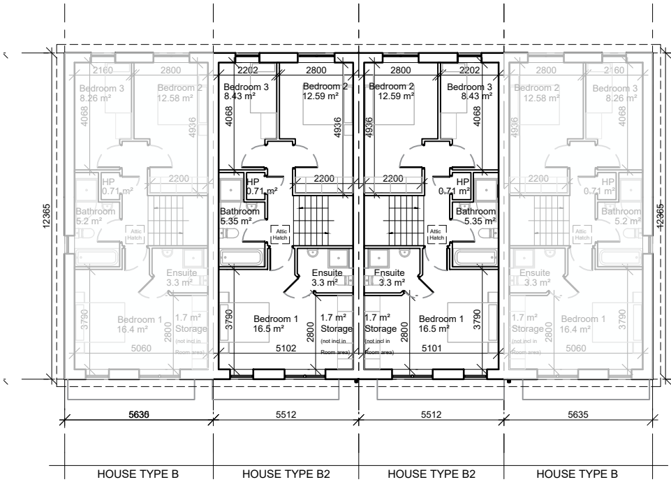
2 First Floor Plan
