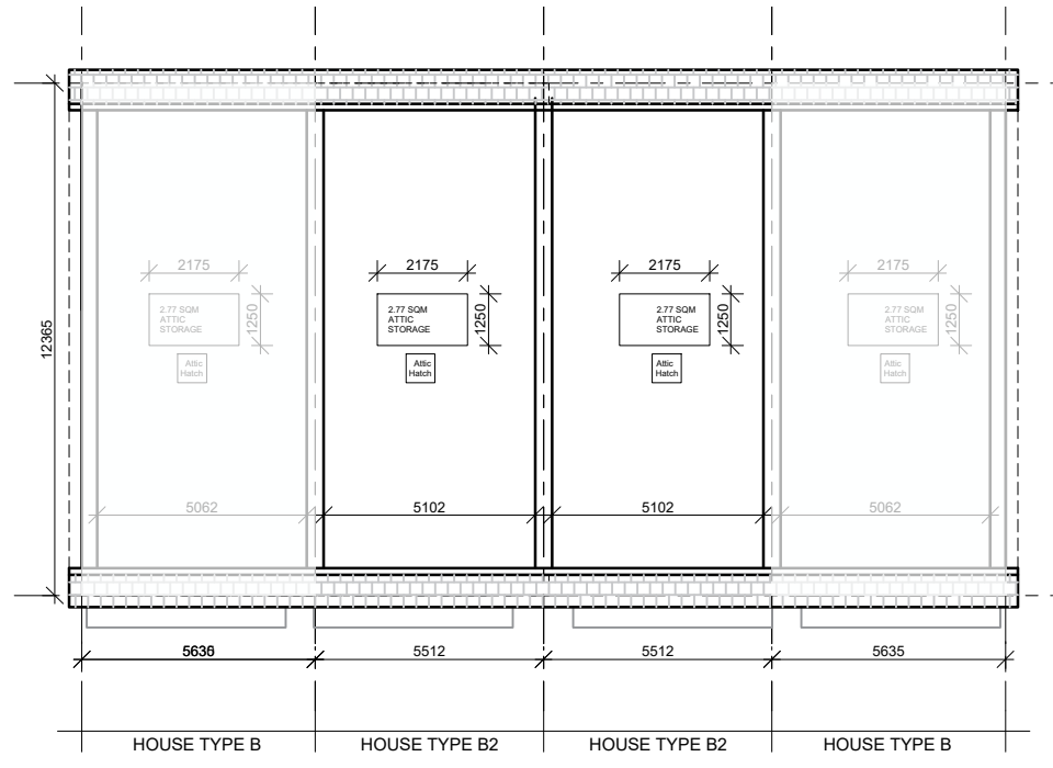
3 First Floor Plan
