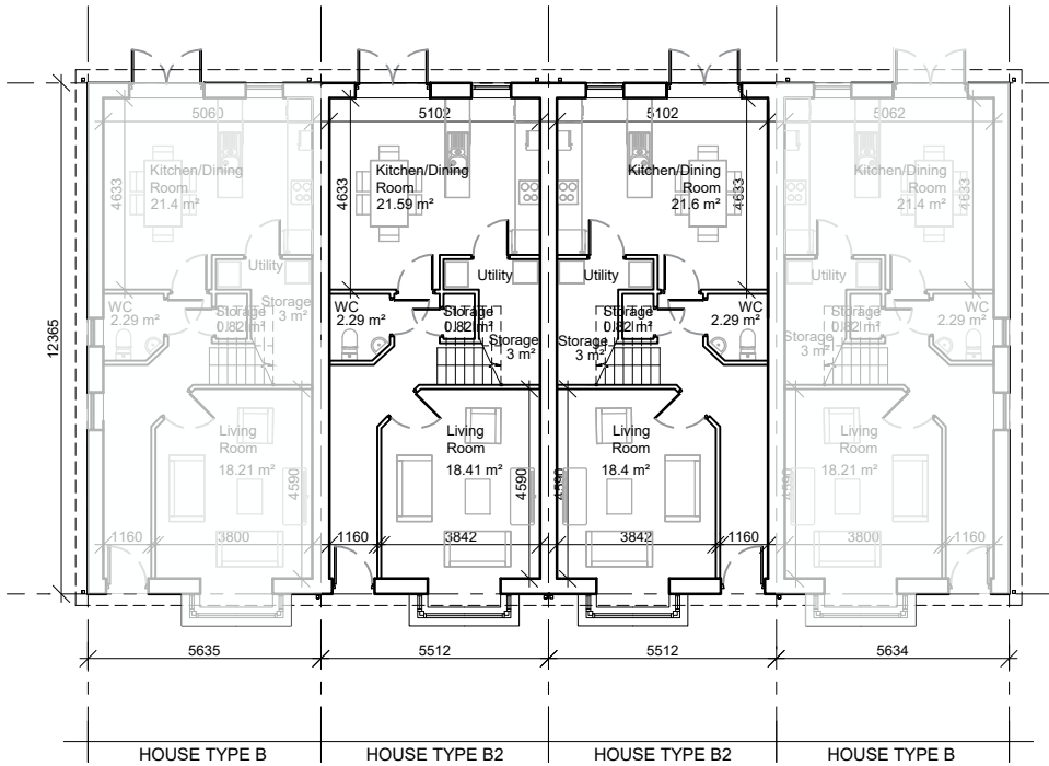
1 Ground Floor Plan
